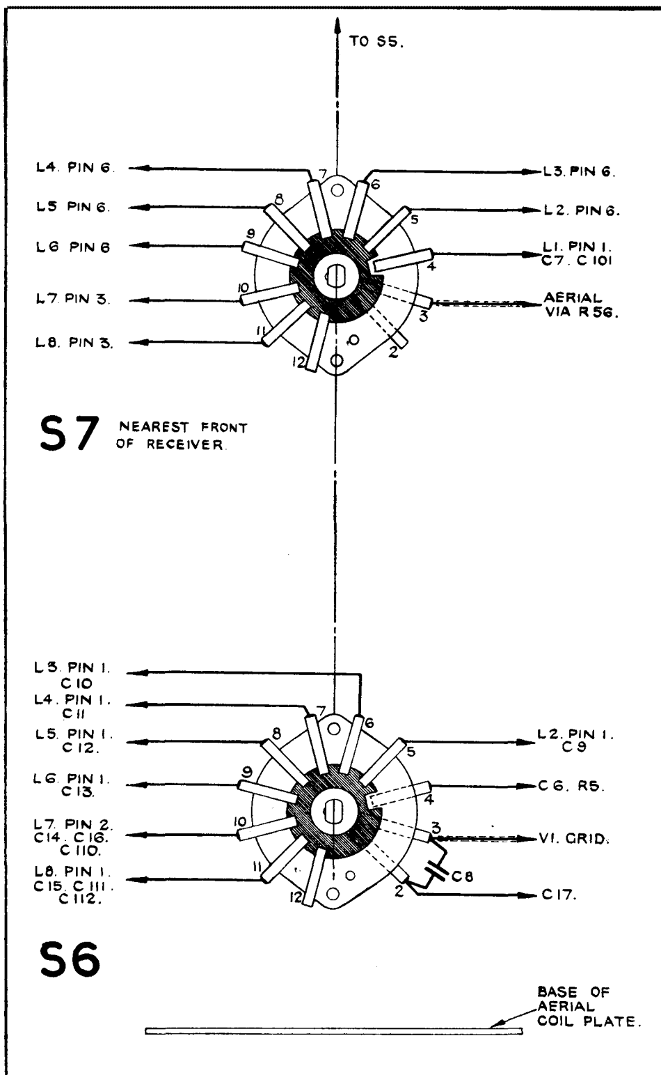
ROTARY SWITCH CONNECTIONS. (View from rear of receiver on underside.)
