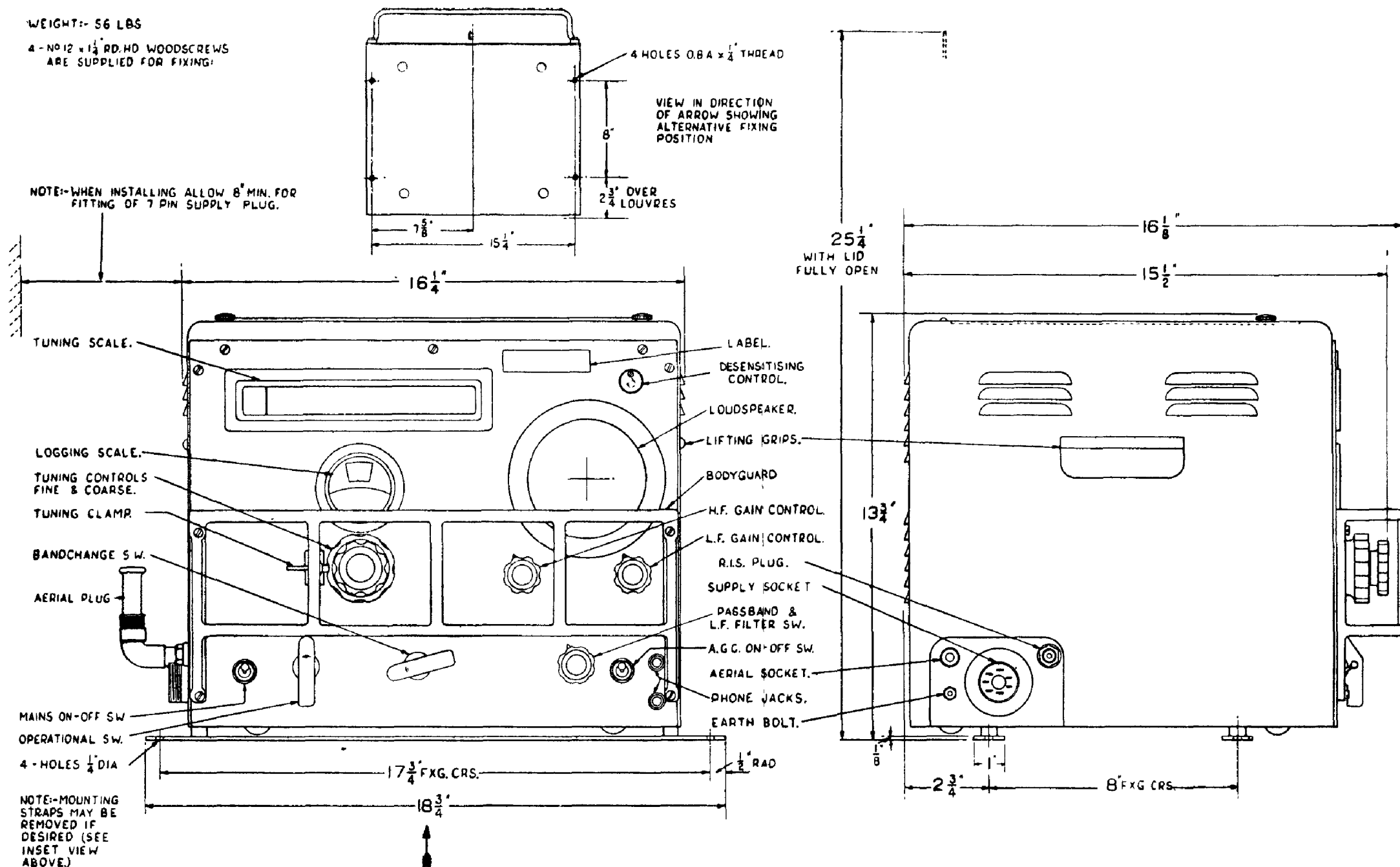
DIMENSIONS OF RECEIVER TYPES CR 300/1 AND CR. 300/2
