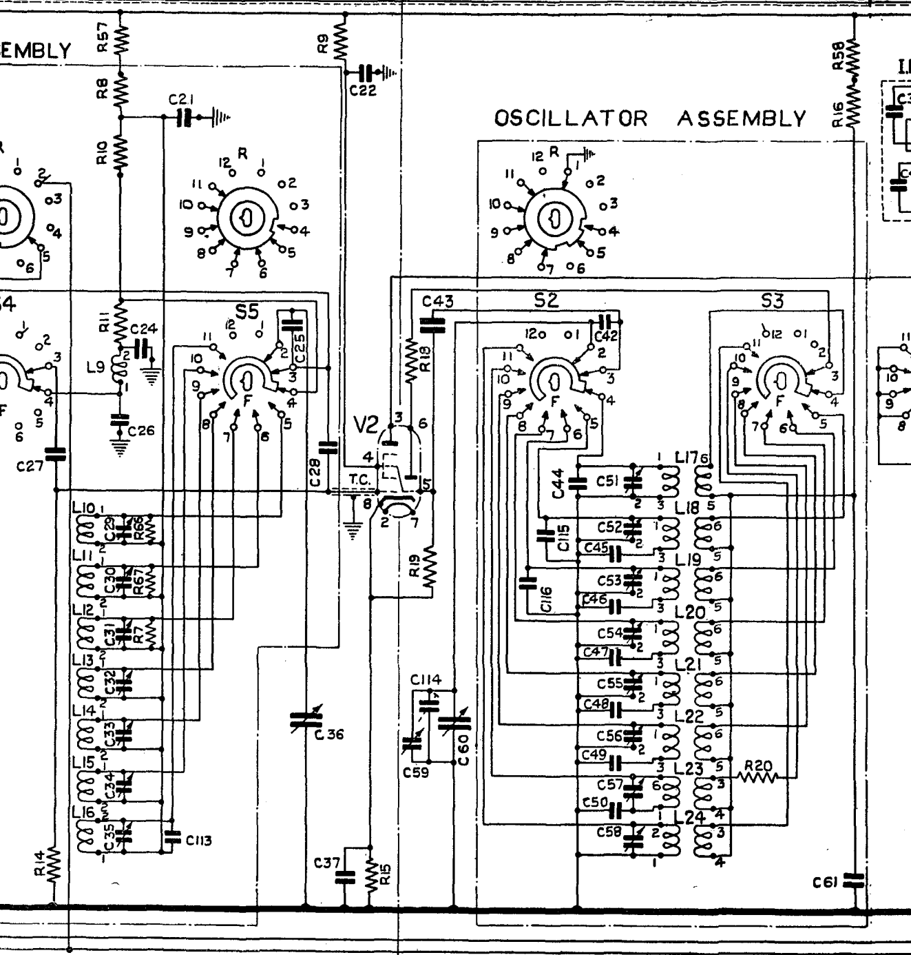
CIRCUIT DIAGRAM OF TYPE CR
