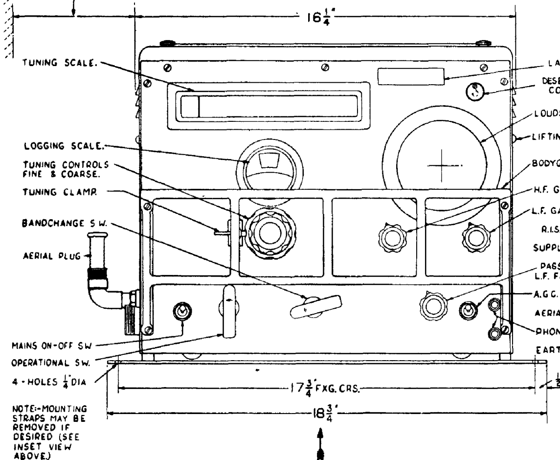
DIMENSIONS OF RECEIVER TYPES C
