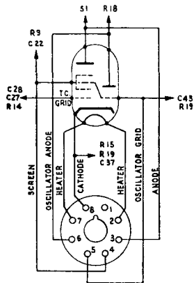
V.2 6K8 or X66. TRIODE - HEXODE FREQUENCY CHANGER.
